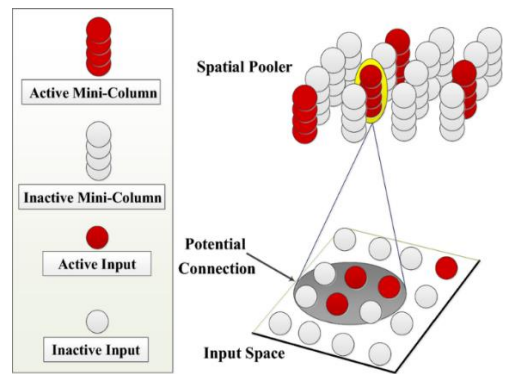
Fig.6: Spatial pooler-algorithm [9]
