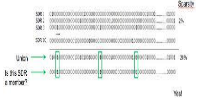
Fig.1: SDR Representation [6]
